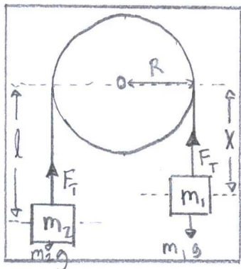
"Atwood machine"
